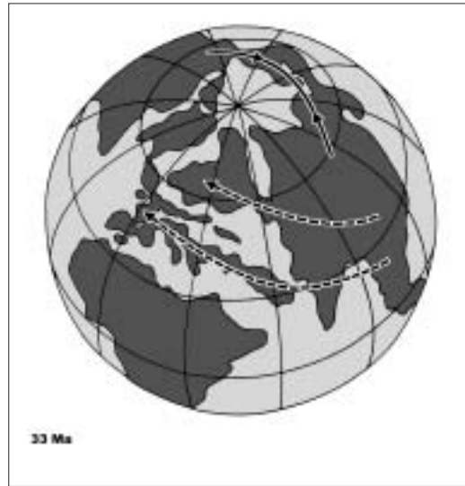
Map 2 Early Oligocene (33MA) continental positions; arrows indicate directions of rodent migrations. The rodent record suggests the proximity of India to Asia and more possibilities of island hopping in the northern Tethys.
