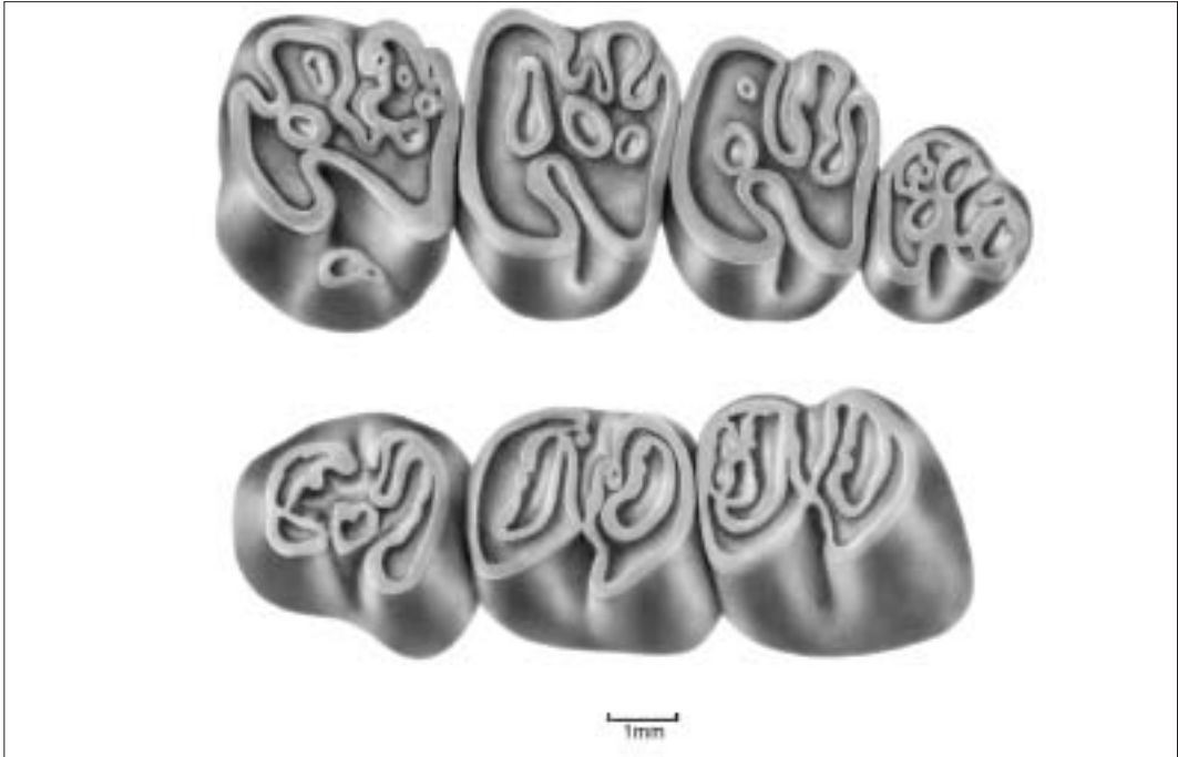
Figure 15 Family Castoridae: Steneofiber butselensis , Hoogbutsel-Hoeleden, Belgium, lower Oligocene (MP21). Occlusal view of above, P4-M3 and below, p4-m2 (after Hugueney 1975).
