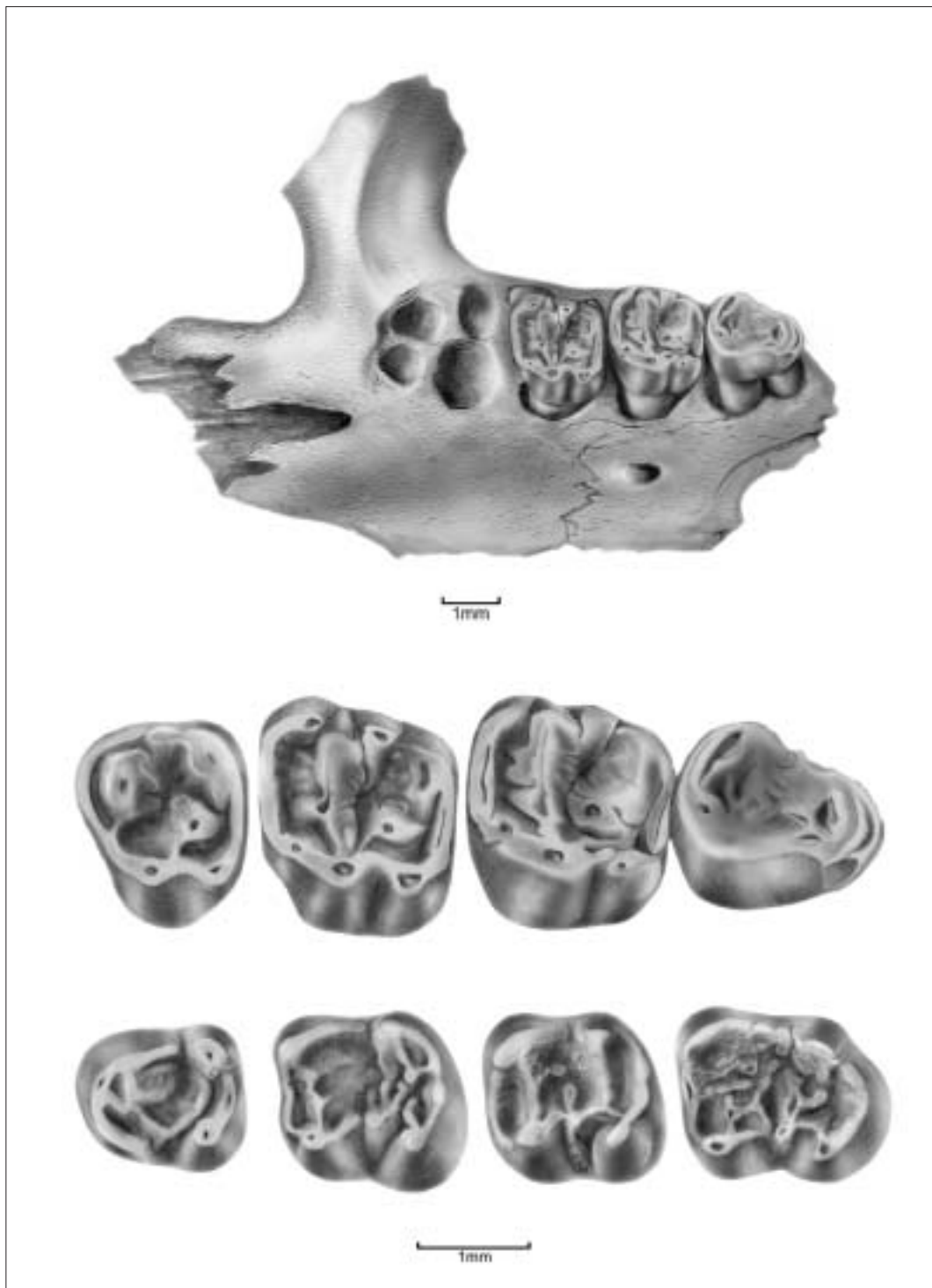
Figure 4 Family Ischyromyidae: Pantogna marandati , Prémontré, France, lower Eocene (MP10). Occlusal views of above, maxilla with M1-3; center, P4-M3; and below p4-m3 (after Escarguel 1999).
