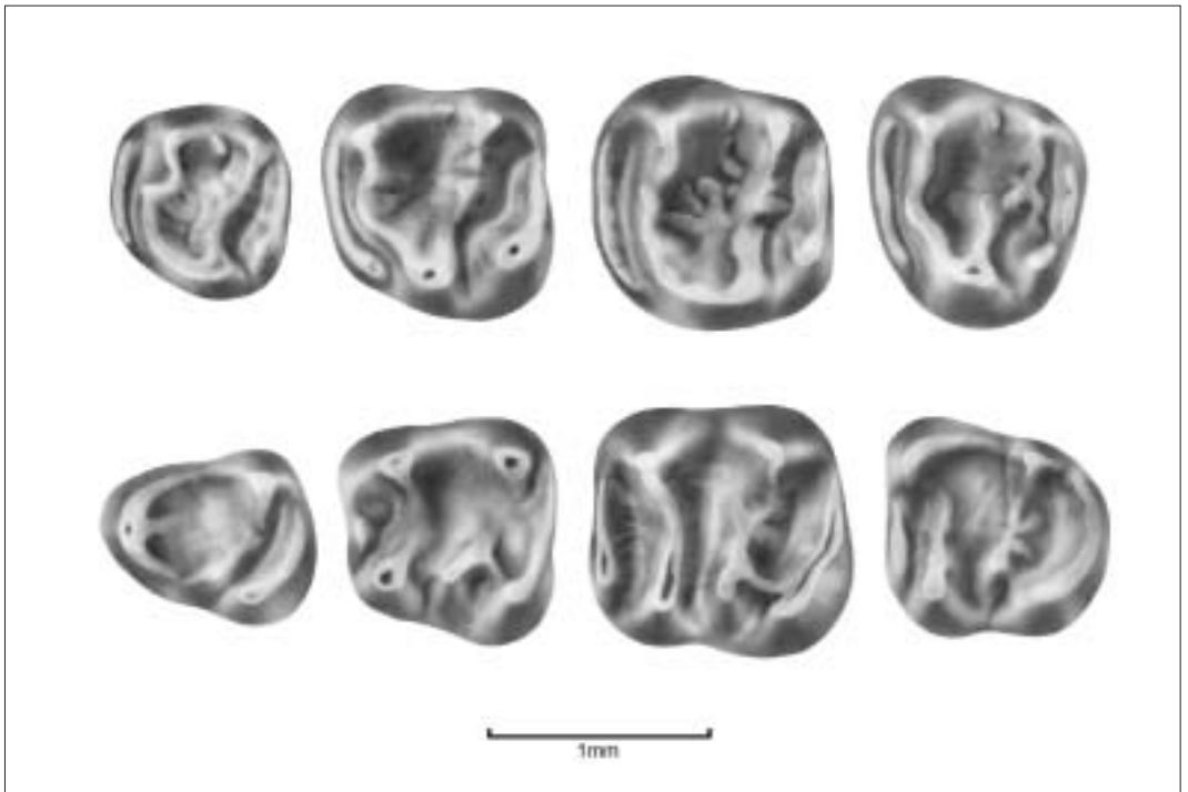
Figure 6 Family Gliiridae: Eogliravus hammeli , Bouxwiller, France, Middle Eocene (MP13). Occlusal views of above, P4-M3 and below, p4-m3 (after Hartenberger 1971).
