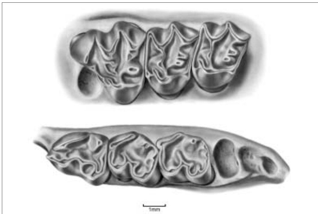
Figure 12 Family Aplodontidae: Plesispermophilus emii , Coderet, France, Upper Oligocene (MP30). Occlusal view of above, maxilla with P4-M2 and below, mandible with p4-m2 (after Viret & Casoli, 1961).
