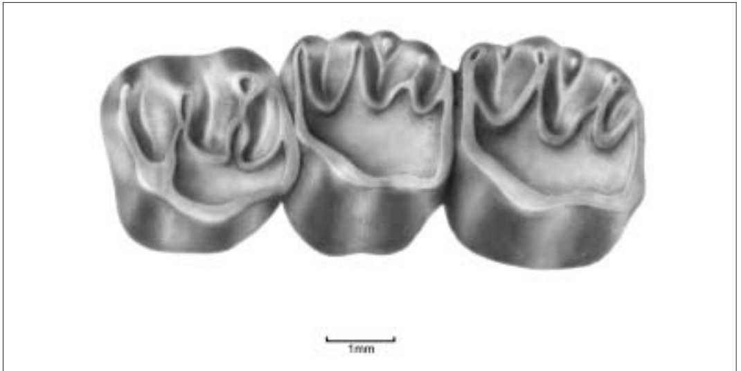
Figure 5 Family Cylindrodontidae: Orientocylindrodon liguanqiaoensis , Shipigou fauna, China, Irдинmanhan. Occlusal view of P4-M2 (after Tong 1997).
