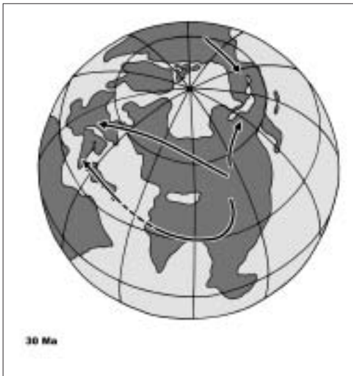
Map 3 Later Oligocene (30Ma) continental positions; arrows indicate direction of rodent migrations.
