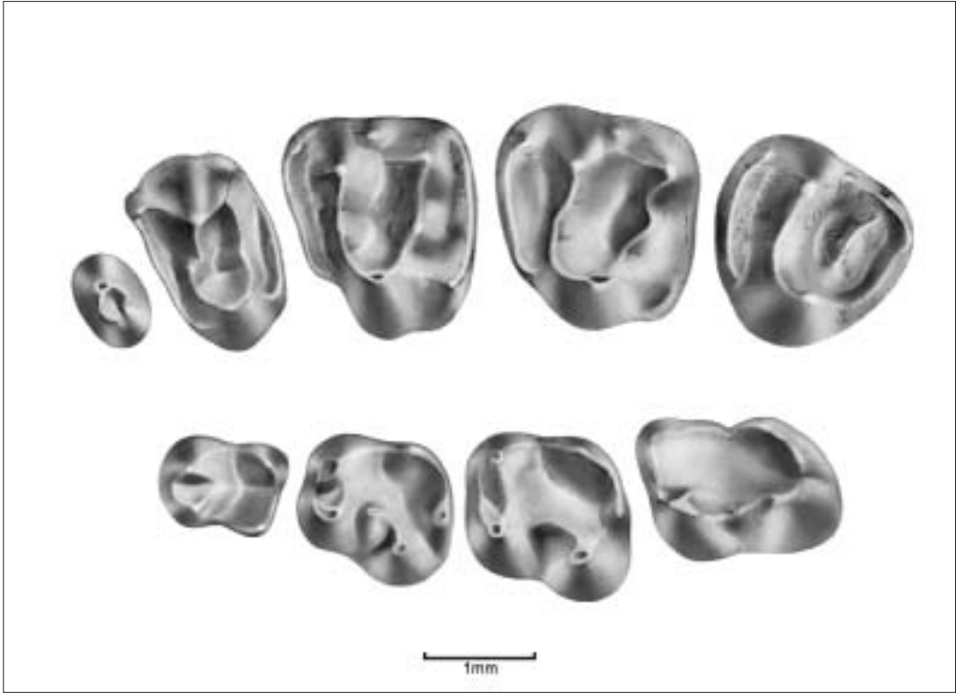
Figure 2. Family Cocomyidae: Cocomys lingchaensis , Hengdong fauna, China, Bumbanian. Occlusal views of above, P3-M3 and below, p4-m3 (after Li et al. 1989).
