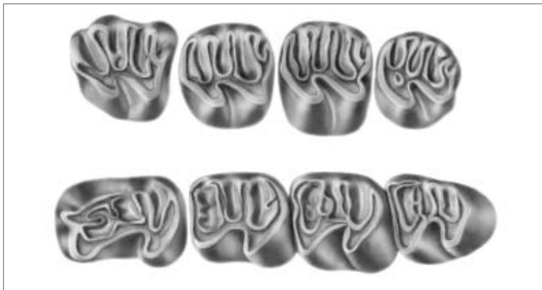
Figure 7 Family Theridomyidae: Theridomys aquatilis , Ronzon, France, lower Oligocene (MP21). Occlusal views of above, P4-M3 and below, p4-m3 (after Vianey-Liaud 1972).
