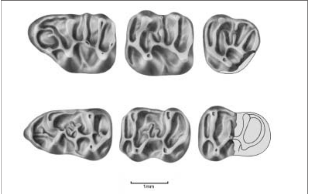
Figure 10 Family Cricetidae: Heterocricetodon hausi , Bumbach, Switzerland, Middle Oligocene (MP25). Occlusal views of above, M1-3 and below, m1-3 (after Engesser 1987).
