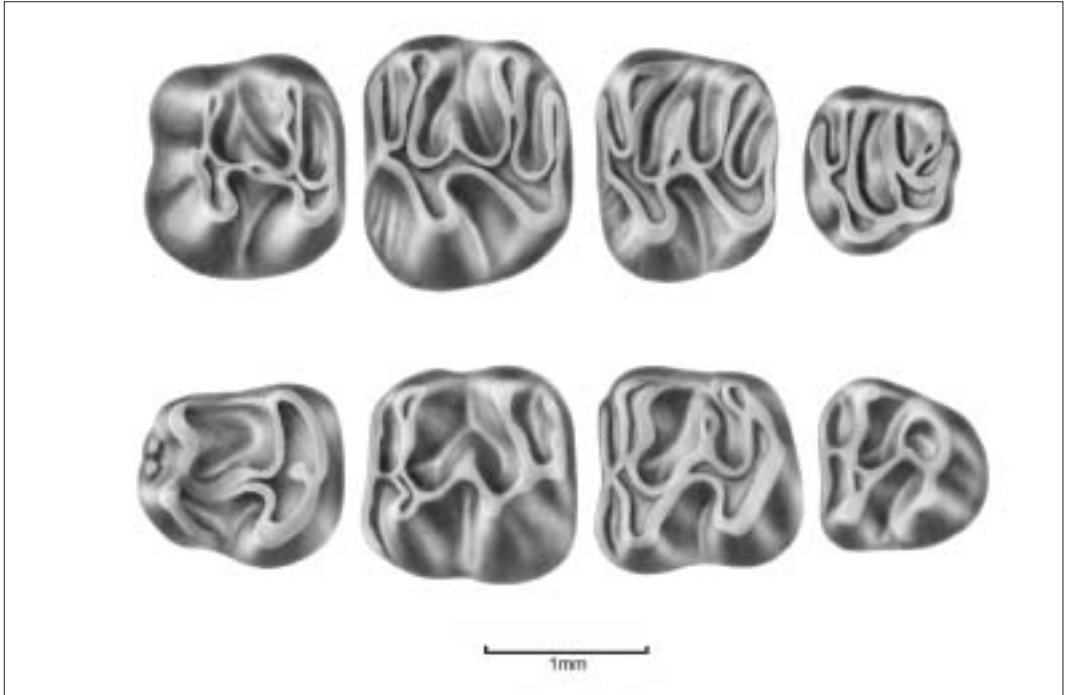
Figure 9 Family Eomyidae: Eomys huerzeleri , Rances, Switzerland, upper Oligocene (MP29). Occlusal views of above, P4-M3 and below, p4-m3 (after Engesser 1999).
