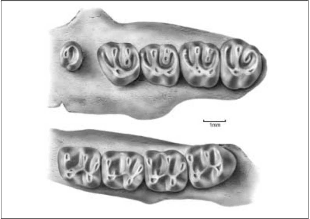
Figure 3 Family Yuomyidae: Yuomys cavioides , Rencun fauna, China, Sharamunian. Occlusal views above, maxilla with P3-M3 and below mandible with p4-m3 (after Li 1975).
