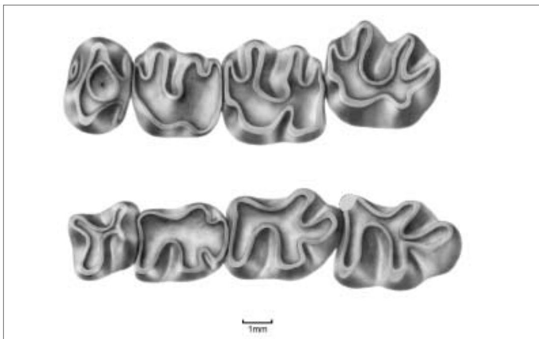
Figure 8 Family Ctenodactylidae: Tataromys plicidens , Hsanda Gol, Mongolia, lower Oligocene, Shandgolian. Occlusal views of above, P4-M3 and below, p4-m3 (after Wang 1997).
