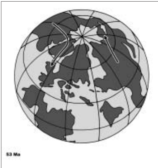
Map 1 Early Eocene (53MA) continental positions; the rodent record supports an interpretation of closer proximity of India to Asia at the time. Arrows indicate directions of rodent migrations. (Sources for map construction: http://www.ods.de/odsn/services/paleomap/paleomap.html (Hay et al. 1999), Heissig 1979b, Smith et al. 1994)
