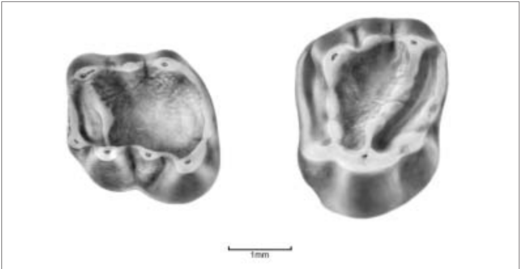
Figure 14 Family Petauristidae: Oligopetes obtusus , Möhren 13, Germany, lower Oligocene (MP22). Occlusal view of left, m1 or 2 and right, M1 or 2 (after Heissig 1979a).
