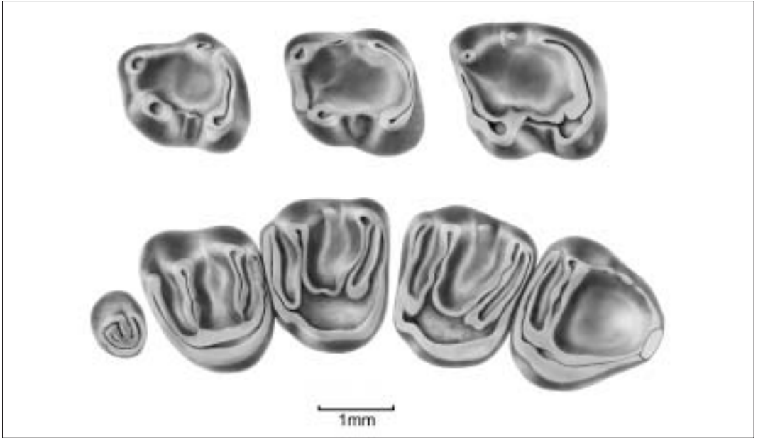
Figure 13 Family Sciuridae: Palaeosciurus goti , Mas de Got, France, lower Oligocene (MP22). Occlusal view of above, p4, m1, m2 and below P3, P4-M3 (after Vianey-Liaud 1974).
