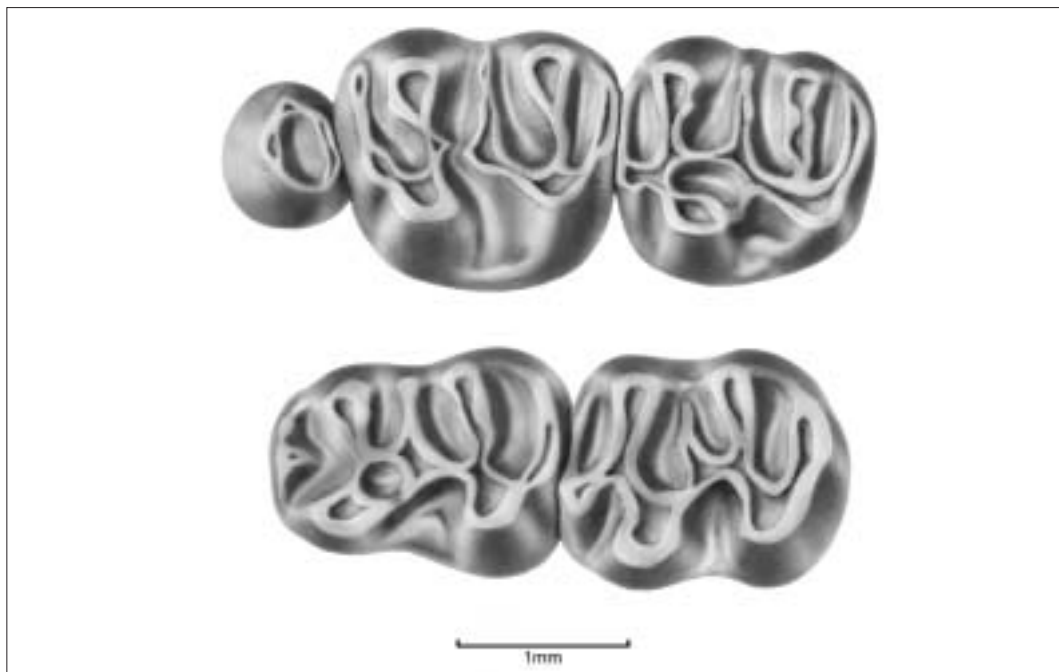
Figure 11 Family Zapodidae: Plesiosminthus schaubi , Coderet, France, Upper Oligocene (MP30). Occlusal view of above, P4-M2 and below, m1-2 (after Engesser 1979).
