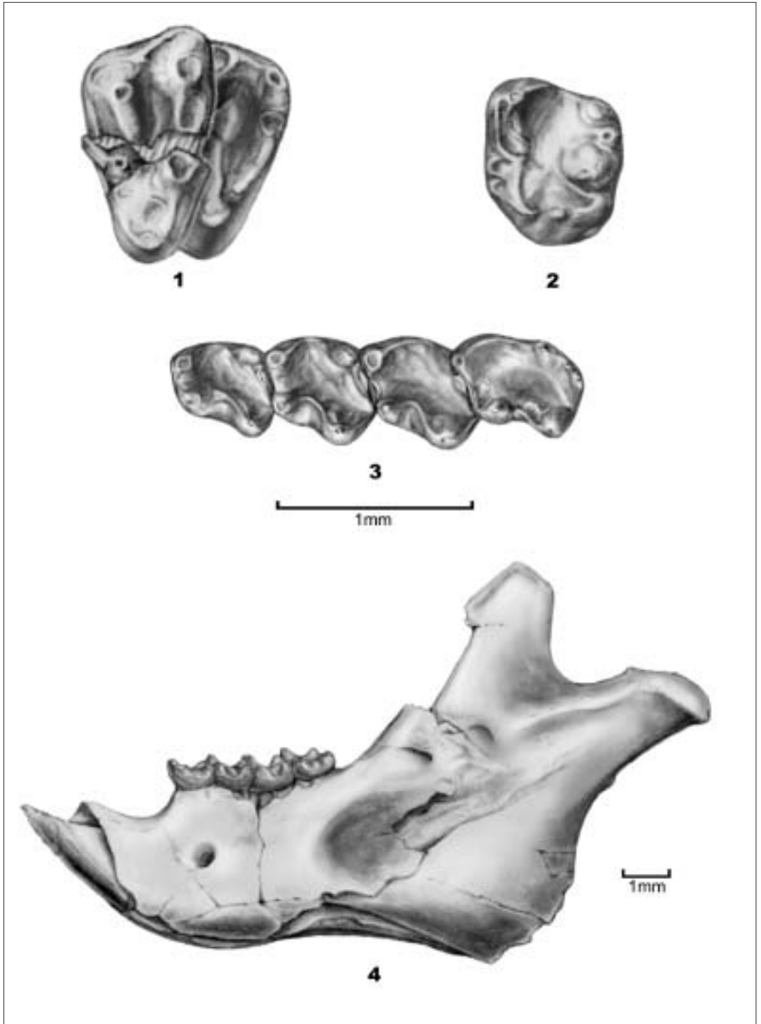
Figure 1 Family Alagomyidae: Alagomys oriensis , Wutu fauna, China, Bumbanian. 1 : occlusal view of M1 overlying M2; 2 : M3; 3 : occlusal view of p4-m3; 4 : lateral view of mandible (after Tong & Dawson 1995). Note: For consistency, all figures have the jaws and teeth positioned to show the upper right side and lower left side.
